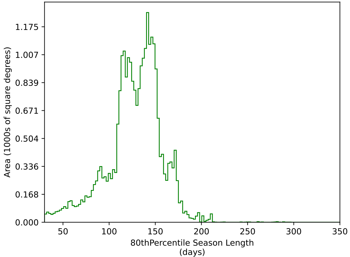
ddf_acor_sf25_lsf40_lsr10_v3.4_10yrs All sky g band: 80thPercentile Season Length
