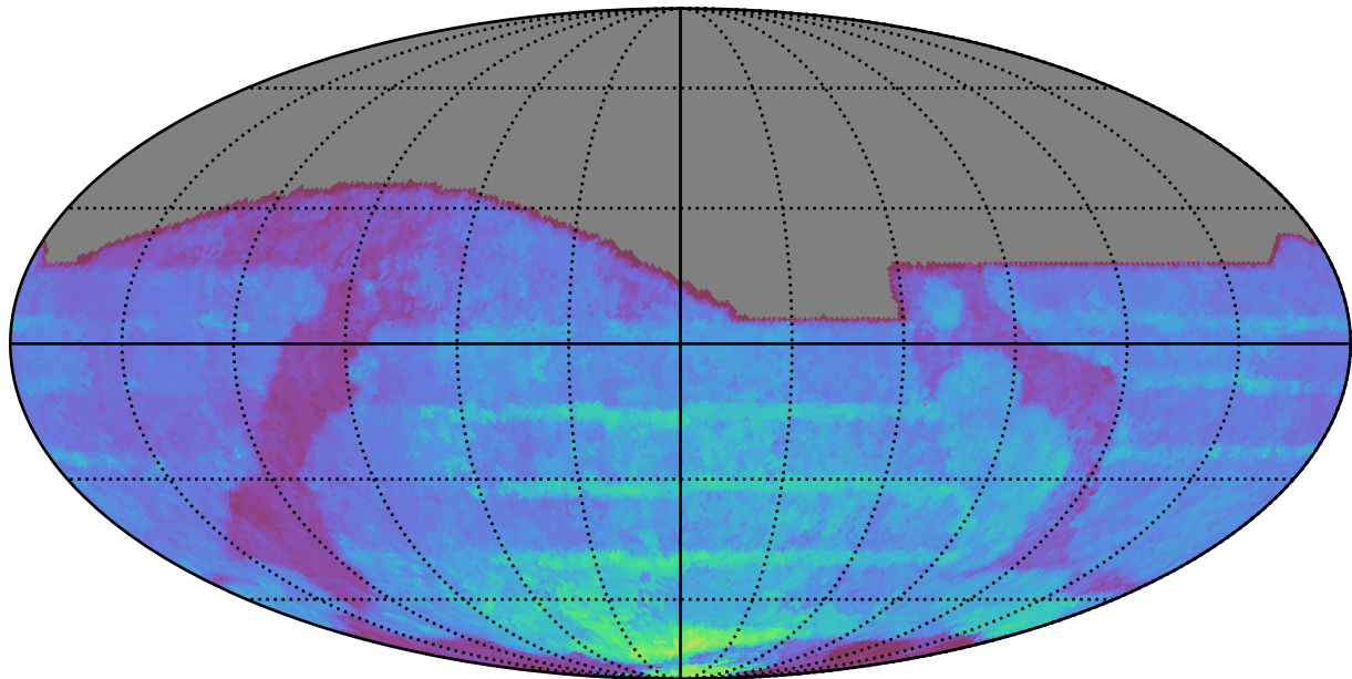
ddf_acor_sf25_lsf40_lsr10_v3.4_10yrs All sky all bands: 80thPercentile Season Length
