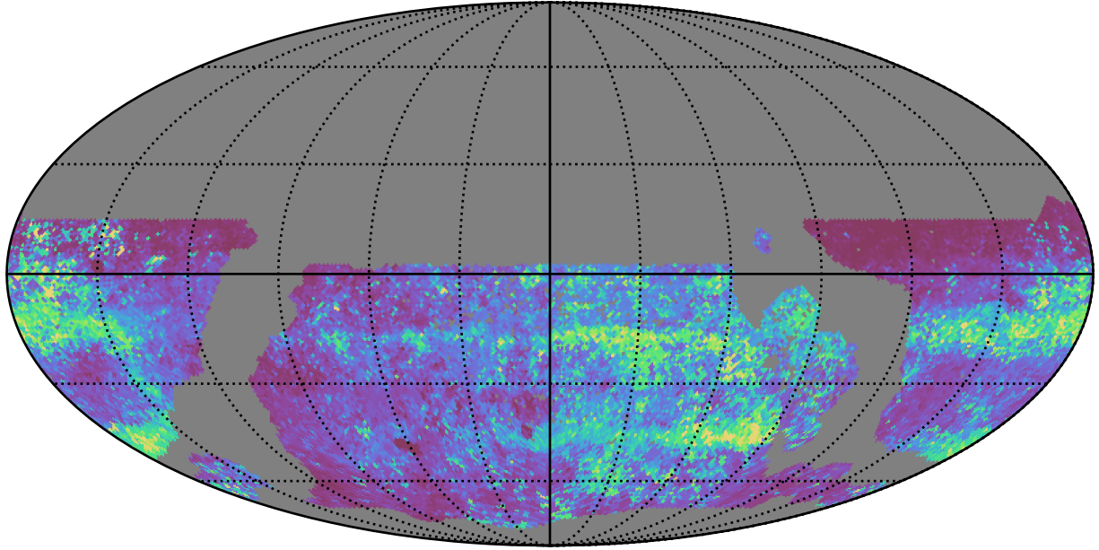
ddf_acor_sf25_lsf40_lsr10_v3.4_10yrs WFD zy bands: 75th Percentile Intranight Timespan
