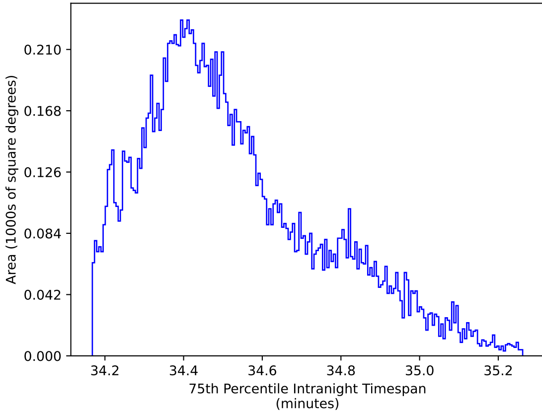
ddf_acor_sf25_lsf40_lsr10_v3.4_10yrs WFD zy bands: 75th Percentile Intranight Timespan
