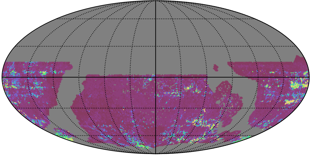
ddf_acor_sf25_lsf40_lsr10_v3.4_10yrs WFD z band: 75th Percentile Intranight Timespan
