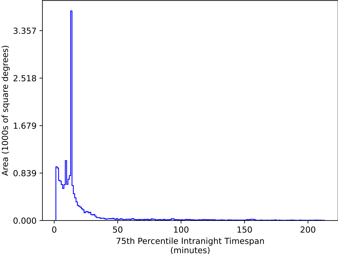
ddf_acor_sf25_lsf40_lsr10_v3.4_10yrs WFD z band: 75th Percentile Intranight Timespan
