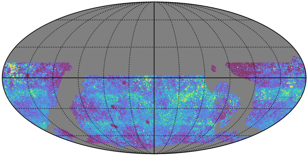
ddf_acor_sf25_lsf40_lsr10_v3.4_10yrs WFD y band: 75th Percentile Intranight Timespan
