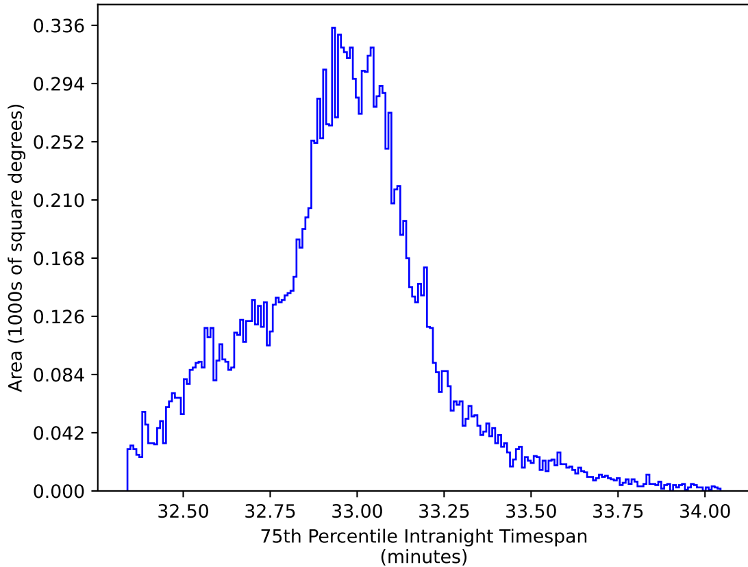
ddf_acor_sf25_lsf40_lsr10_v3.4_10yrs WFD y band: 75th Percentile Intranight Timespan
