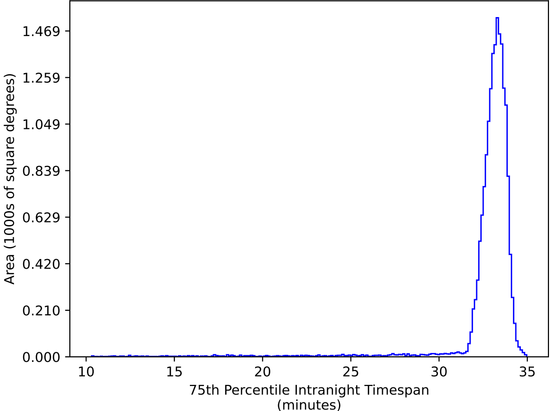
ddf_acor_sf25_lsf40_lsr10_v3.4_10yrs WFD ug bands: 75th Percentile Intranight Timespan
