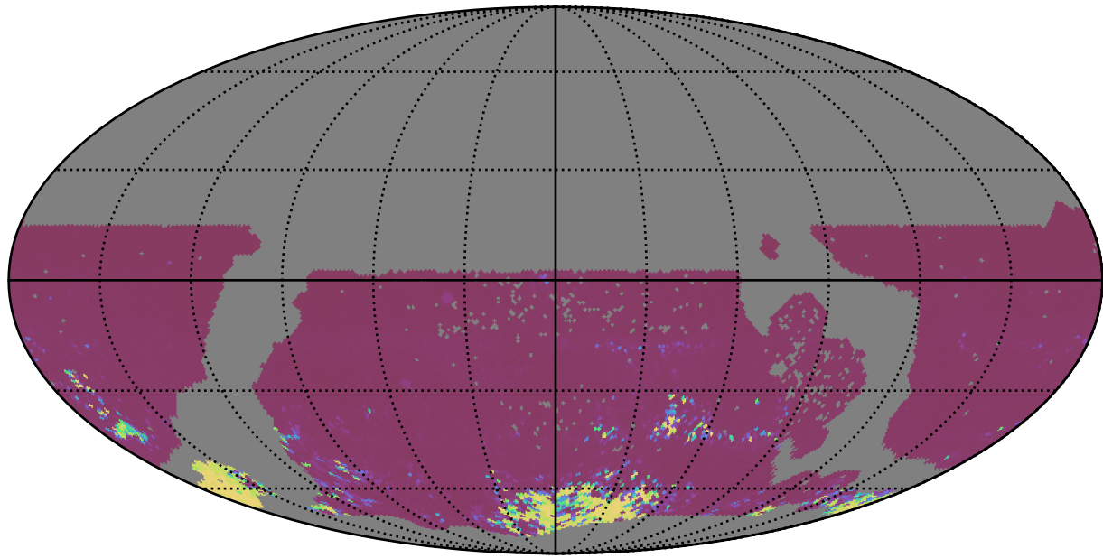
ddf_acor_sf25_lsf40_lsr10_v3.4_10yrs WFD ri bands: 75th Percentile Intranight Timespan
