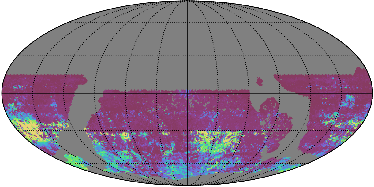
ddf_acor_sf25_lsf40_lsr10_v3.4_10yrs WFD r band: 75th Percentile Intranight Timespan
