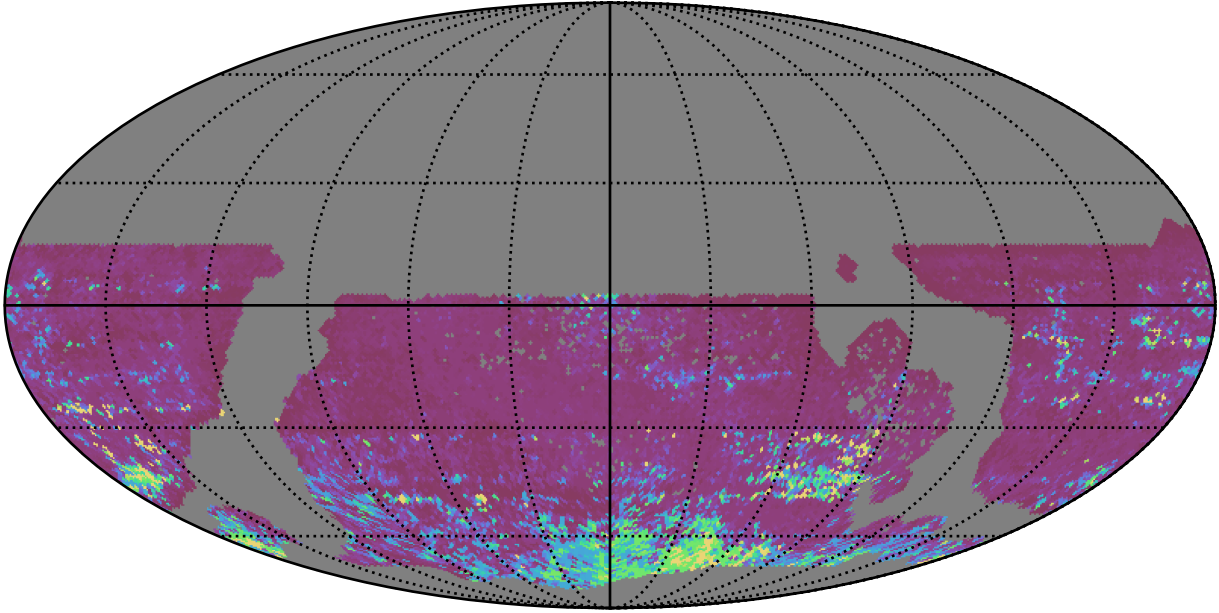
ddf_acor_sf25_lsf40_lsr10_v3.4_10yrs WFD i band: 75th Percentile Intranight Timespan
