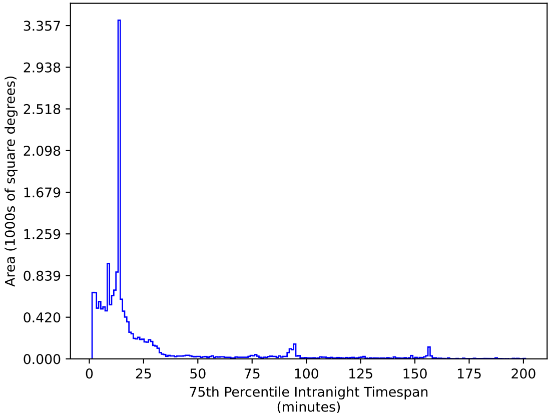
ddf_acor_sf25_lsf40_lsr10_v3.4_10yrs WFD i band: 75th Percentile Intranight Timespan
