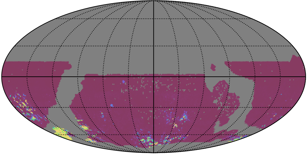
ddf_acor_sf25_lsf40_lsr10_v3.4_10yrs WFD gr bands: 75th Percentile Intranight Timespan
