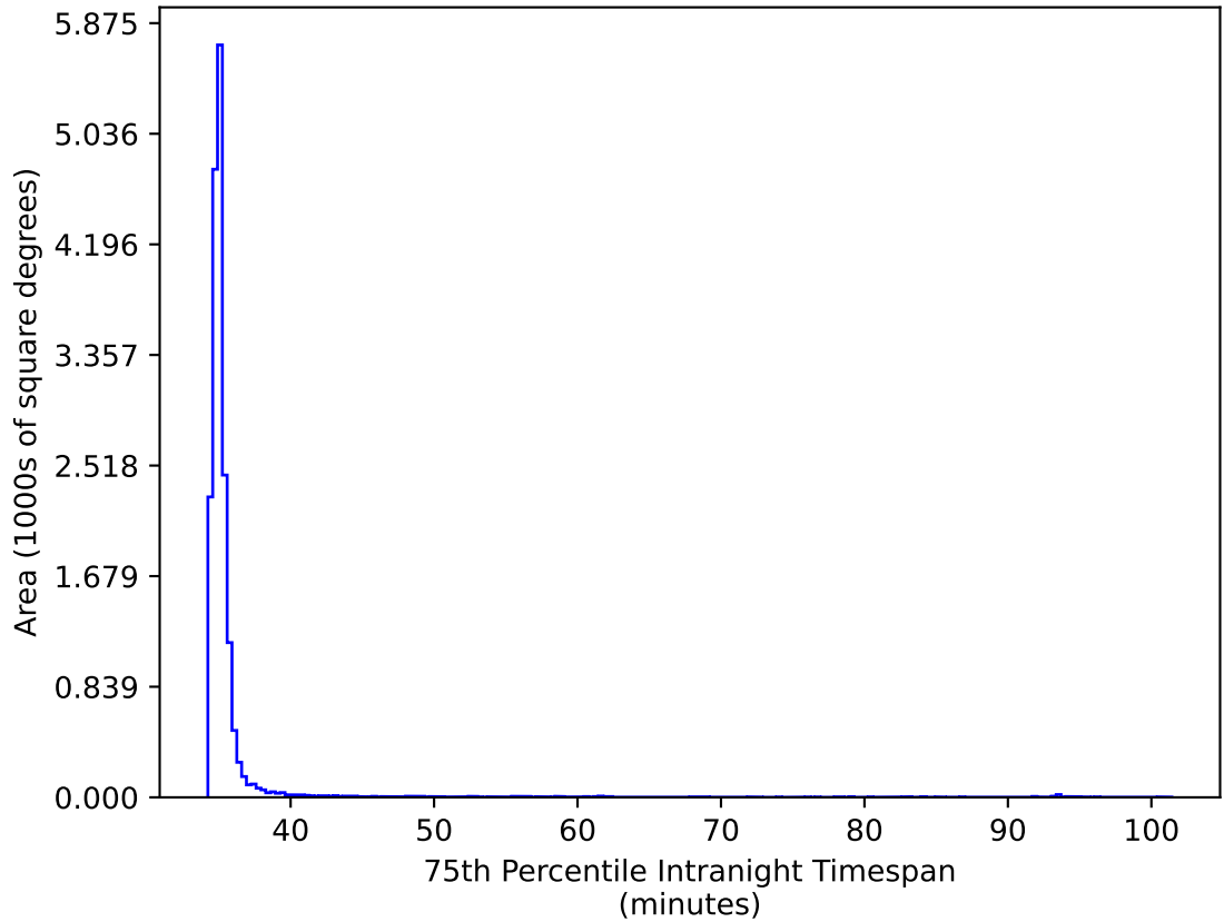
ddf_acor_sf25_lsf40_lsr10_v3.4_10yrs WFD gr bands: 75th Percentile Intranight Timespan
