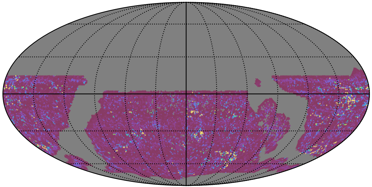
ddf_acor_sf25_lsf40_lsr10_v3.4_10yrs WFD g band: 75th Percentile Intranight Timespan
