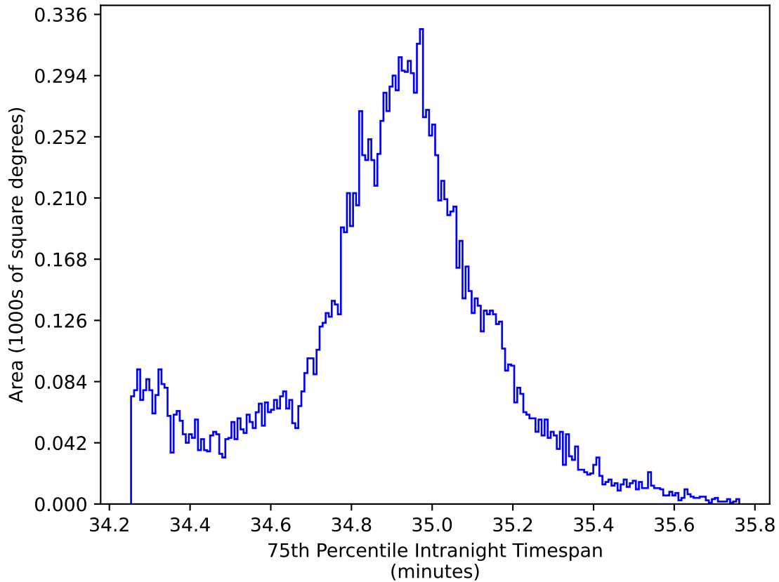
ddf_acor_sf25_Isf40_Isr10_v3.4_10yrs WFD all bands: 75th Percentile Intranight Timespan
