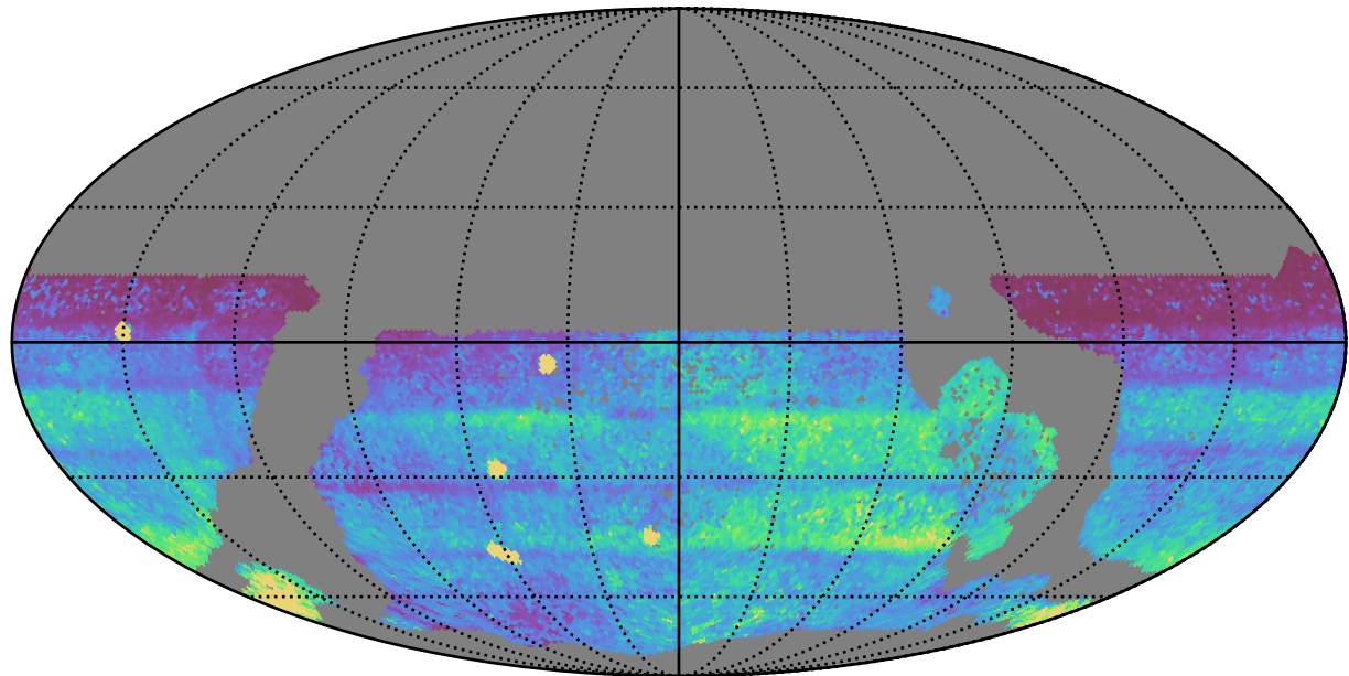
ddf_acor_sf25_lsf40_lsr10_v3.4_10yrs WFD: 75th Percentile Intranight Timespan
