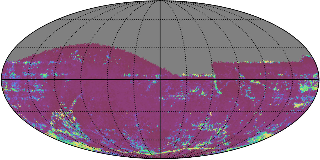
ddf_acor_sf25_lsf40_lsr10_v3.4_10yrs All sky z band: 75th Percentile Intranight Timespan
