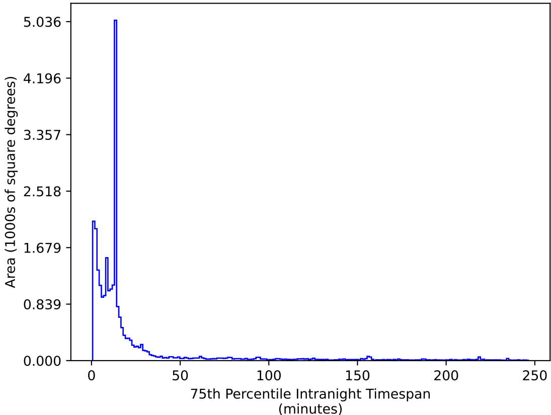
ddf_acor_sf25_lsf40_lsr10_v3.4_10yrs All sky z band: 75th Percentile Intranight Timespan
