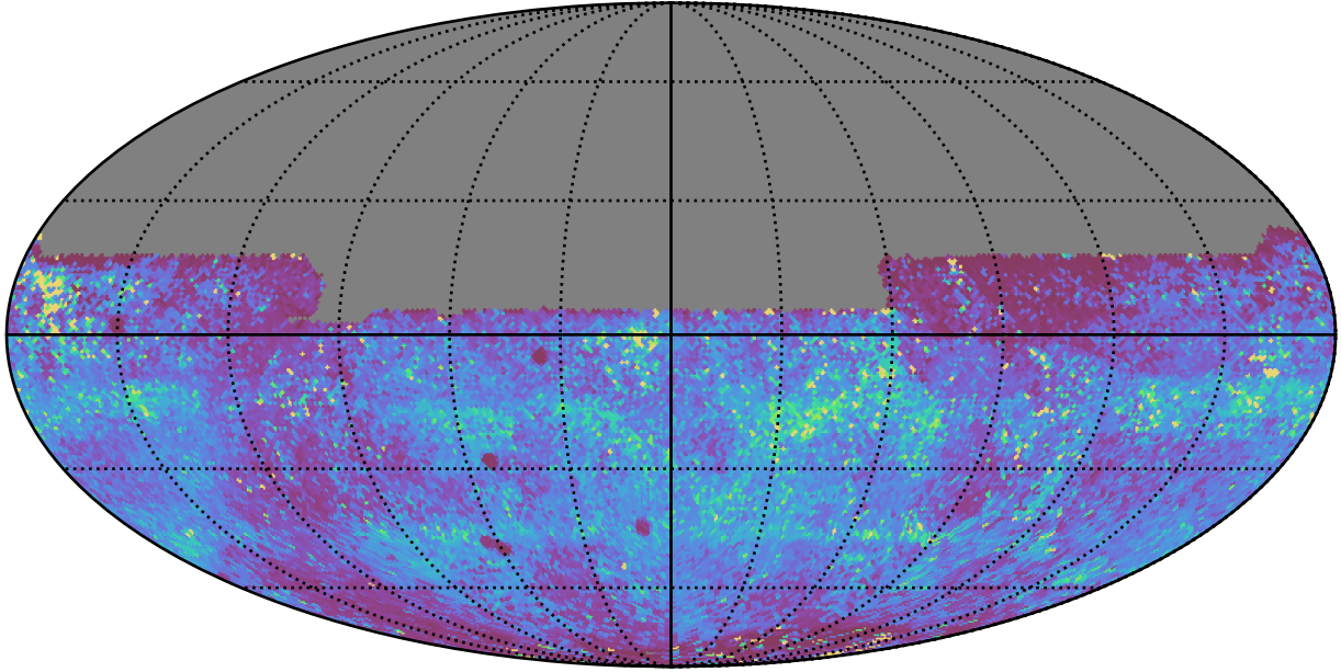
ddf_acor_sf25_lsf40_lsr10_v3.4_10yrs All sky y band: 75th Percentile Intranight Timespan
