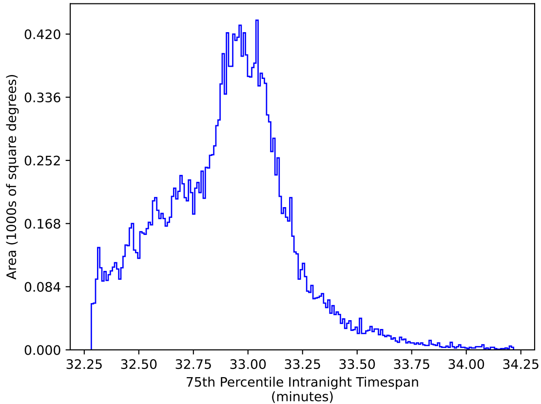
ddf_acor_sf25_ls40_lsr10_v3.4_10yrs All sky y band: 75th Percentile Intranight Timespan
