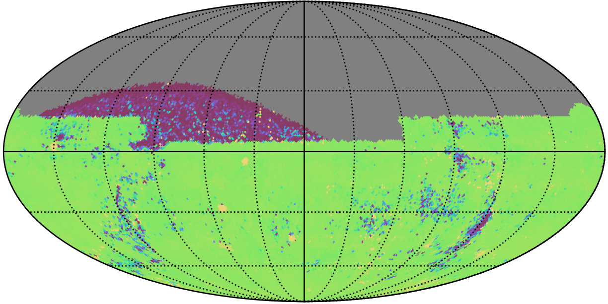
ddf_acor_sf25_lsf40_lsr10_v3.4_10yrs All sky ug bands: 75th Percentile Intranight Timespan
