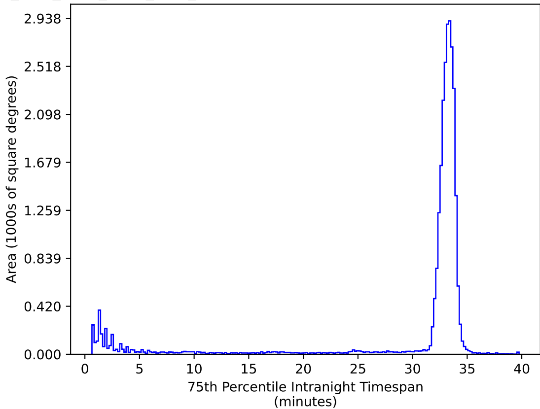
ddf_acor_sf25_lsf40_lsr10_v3.4_10yrs All sky ug bands: 75th Percentile Intranight Timespan
