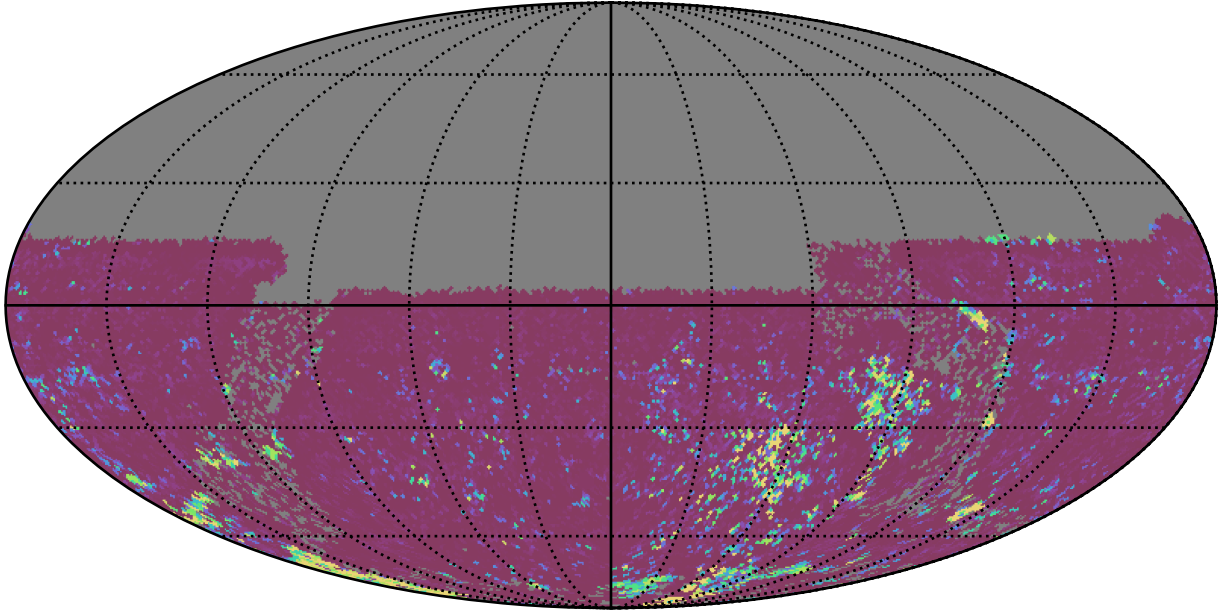
ddf_acor_sf25_lsf40_lsr10_v3.4_10yrs All sky u band: 75th Percentile Intranight Timespan
