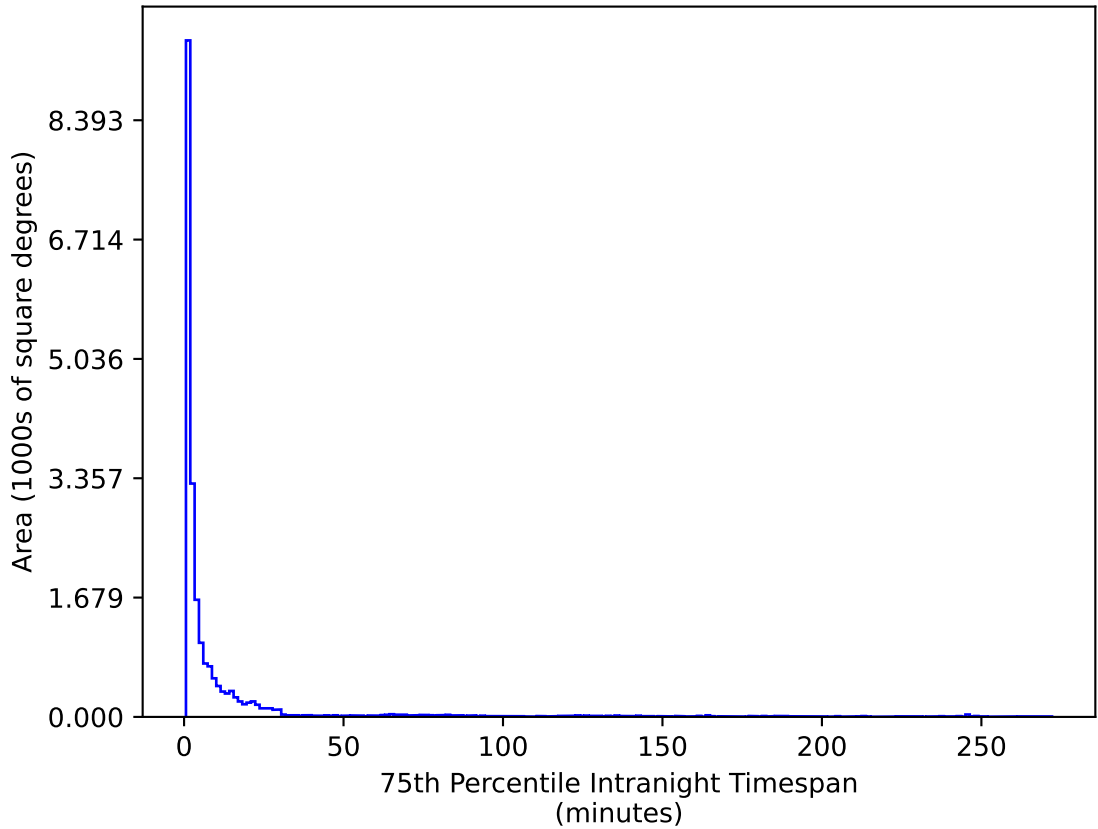
ddf_acor_sf25_lsf40_lsr10_v3.4_10yrs All sky u band: 75th Percentile Intranight Timespan
