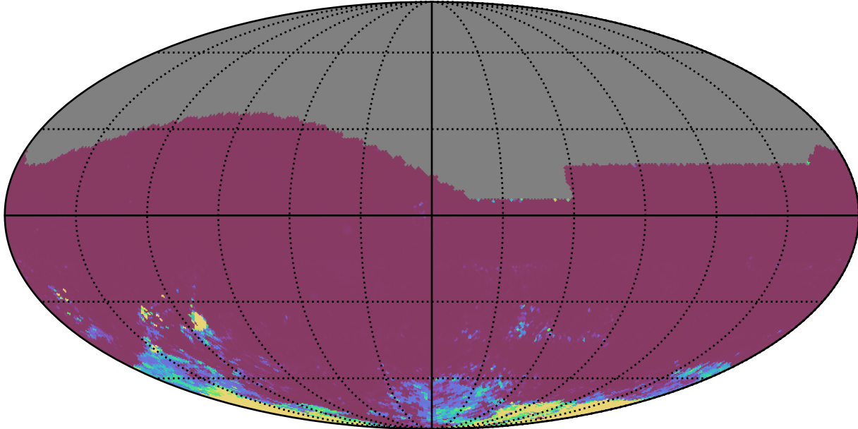
ddf_acor_sf25_lsf40_lsr10_v3.4_10yrs All sky ri bands: 75th Percentile Intranight Timespan
