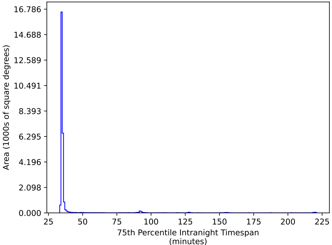
ddf_acor_sf25_lsf40_lsr10_v3.4_10yrs All sky ri bands: 75th Percentile Intranight Timespan
