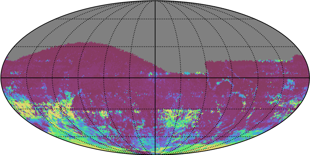
ddf_acor_sf25_lsf40_lsr10_v3.4_10yrs All sky r band: 75th Percentile Intranight Timespan
