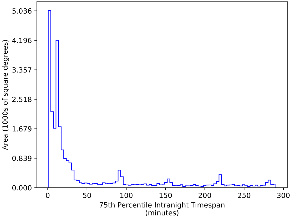
ddf_acor_sf25_lsf40_lsr10_v3.4_10yrs All sky r band: 75th Percentile Intranight Timespan
