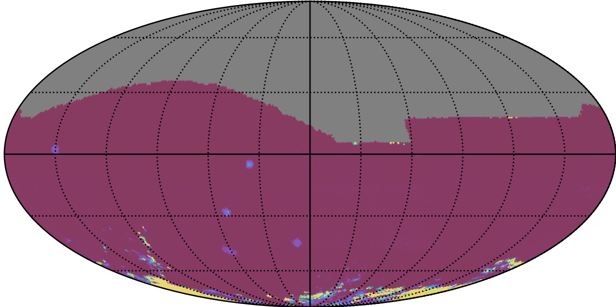
ddf_acor_sf25_lsf40_lsr10_v3.4_10yrs All sky iz bands: 75th Percentile Intranight Timespan
