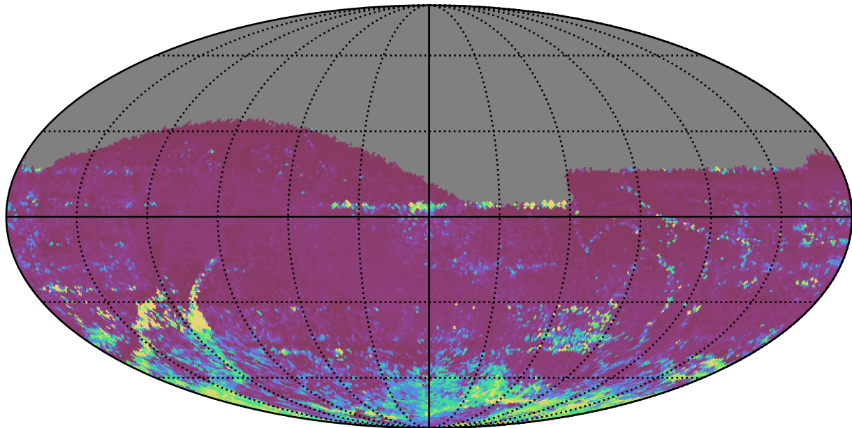
ddf_acor_sf25_lsf40_lsr10_v3.4_10yrs All sky i band: 75th Percentile Intranight Timespan
