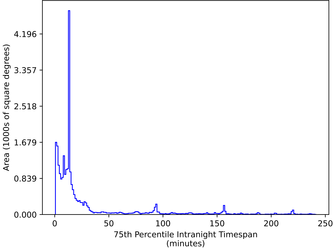
ddf_acor_sf25_lsf40_lsr10_v3.4_10yrs All sky i band: 75th Percentile Intranight Timespan
