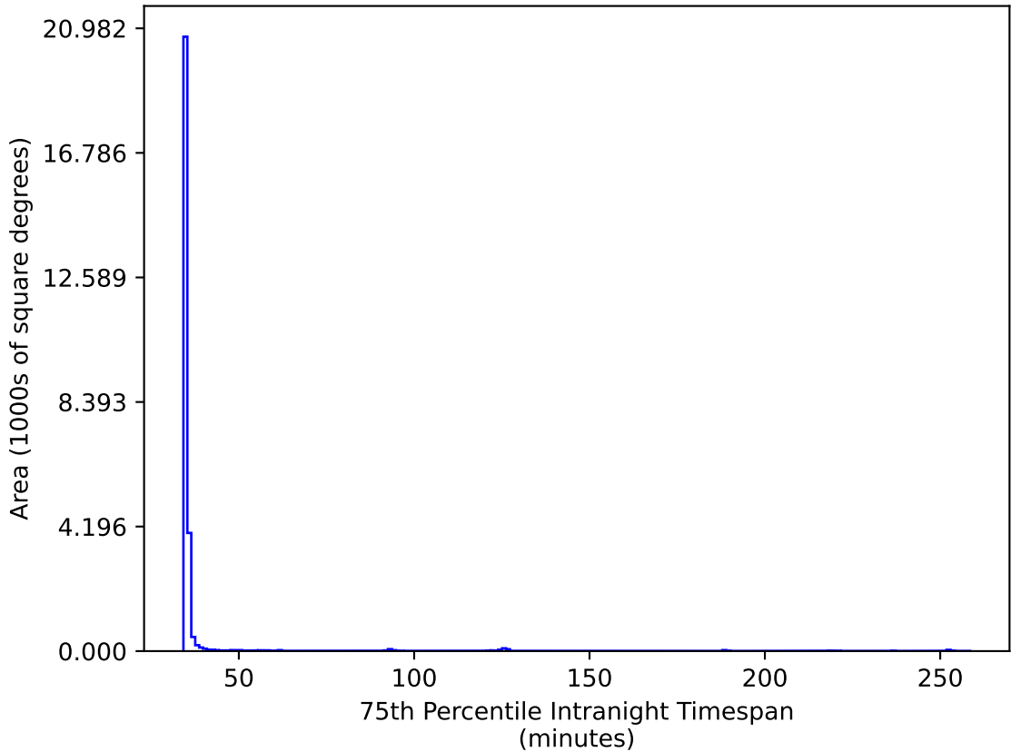
ddf_acor_sf25_lsf40_lsr10_v3.4_10yrs All sky gr bands: 75th Percentile Intranight Timespan
