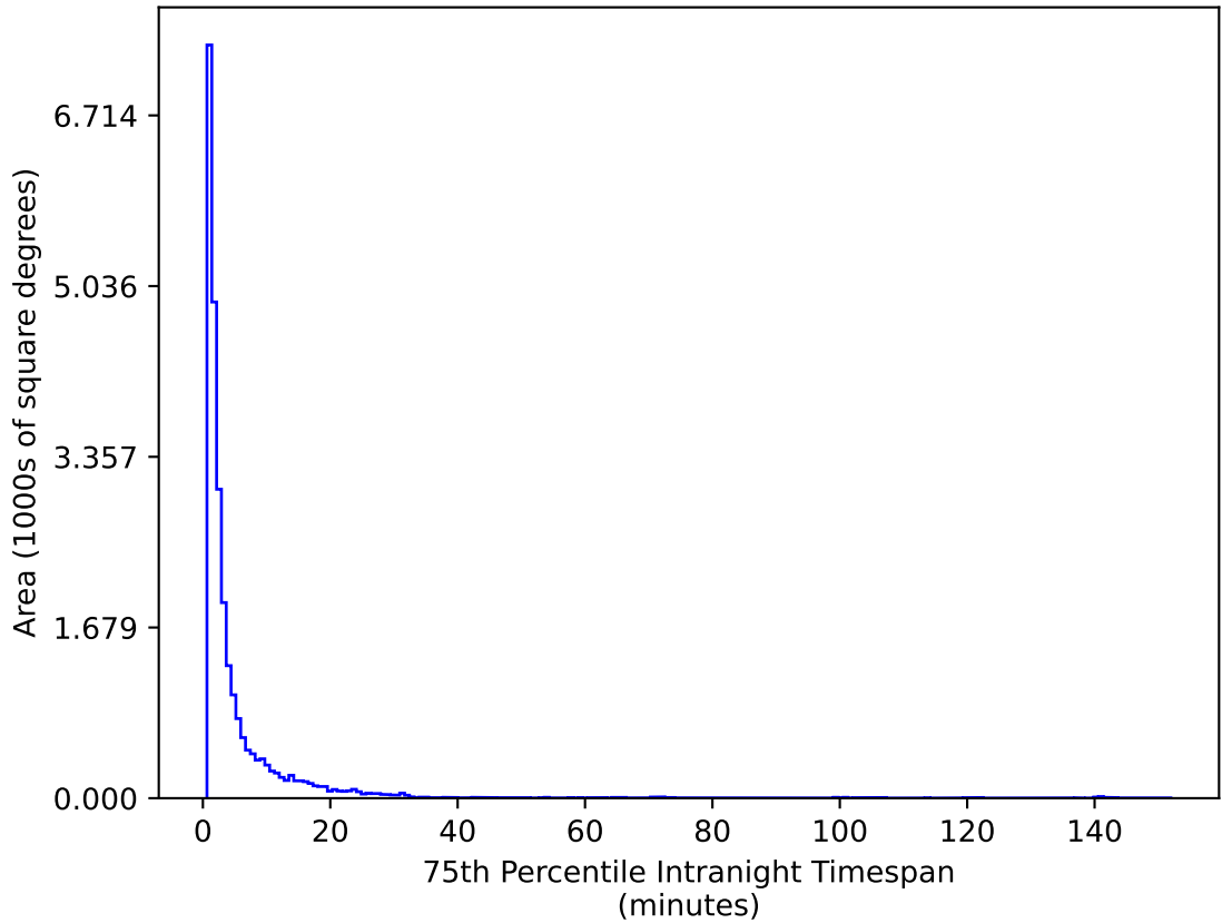
ddf_acor_sf25_lsf40_lsr10_v3.4_10yrs All sky g band: 75th Percentile Intranight Timespan
