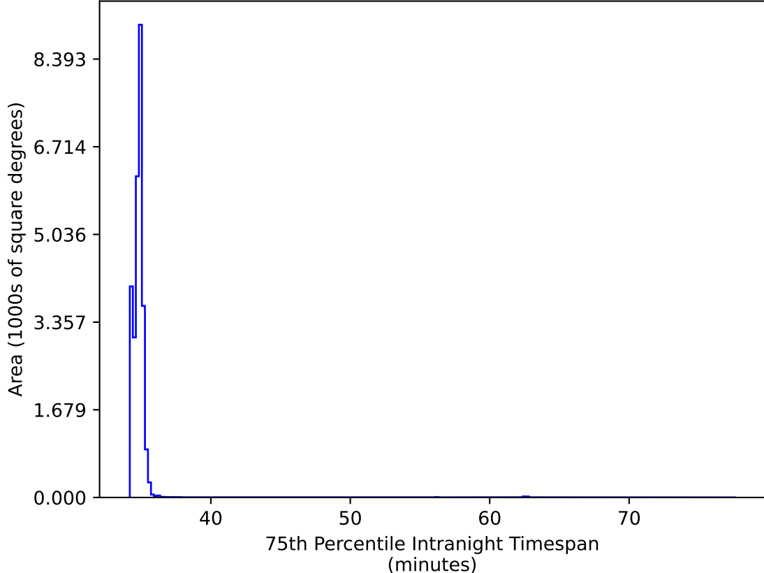
ddf_acor_sf25_lsf40_lsr10_v3.4_10yrs All sky all bands: 75th Percentile Intranight Timespan
