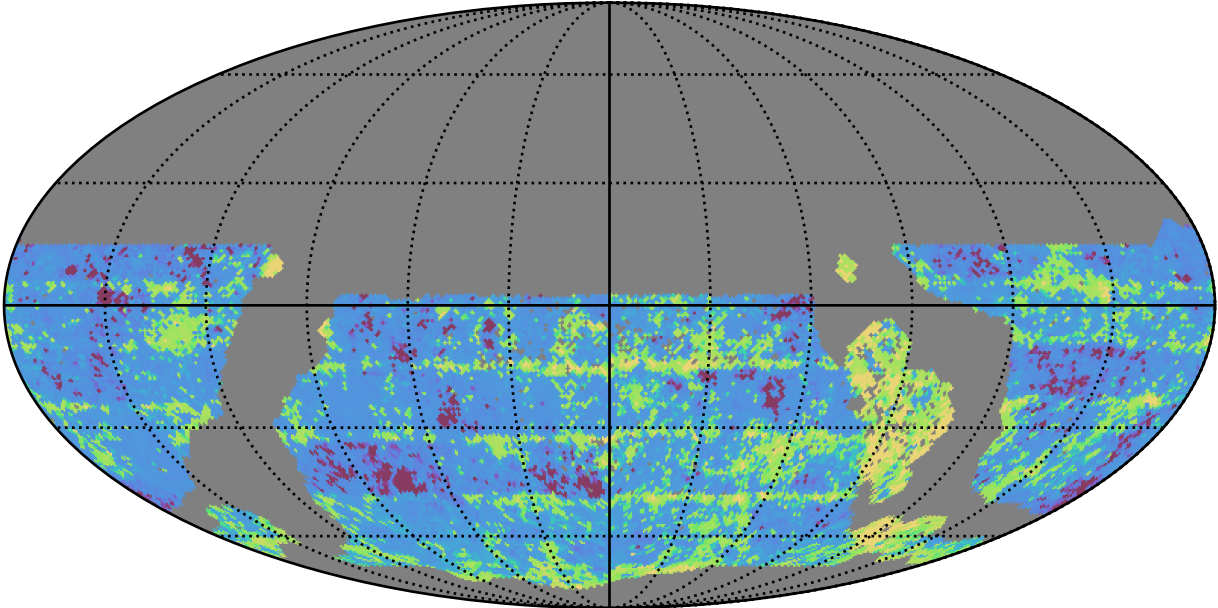
ddf_acor_sf25_lsf40_lsr10_v3.4_10yrs WFD z band: 20thPercentile Inter-Night Gap
