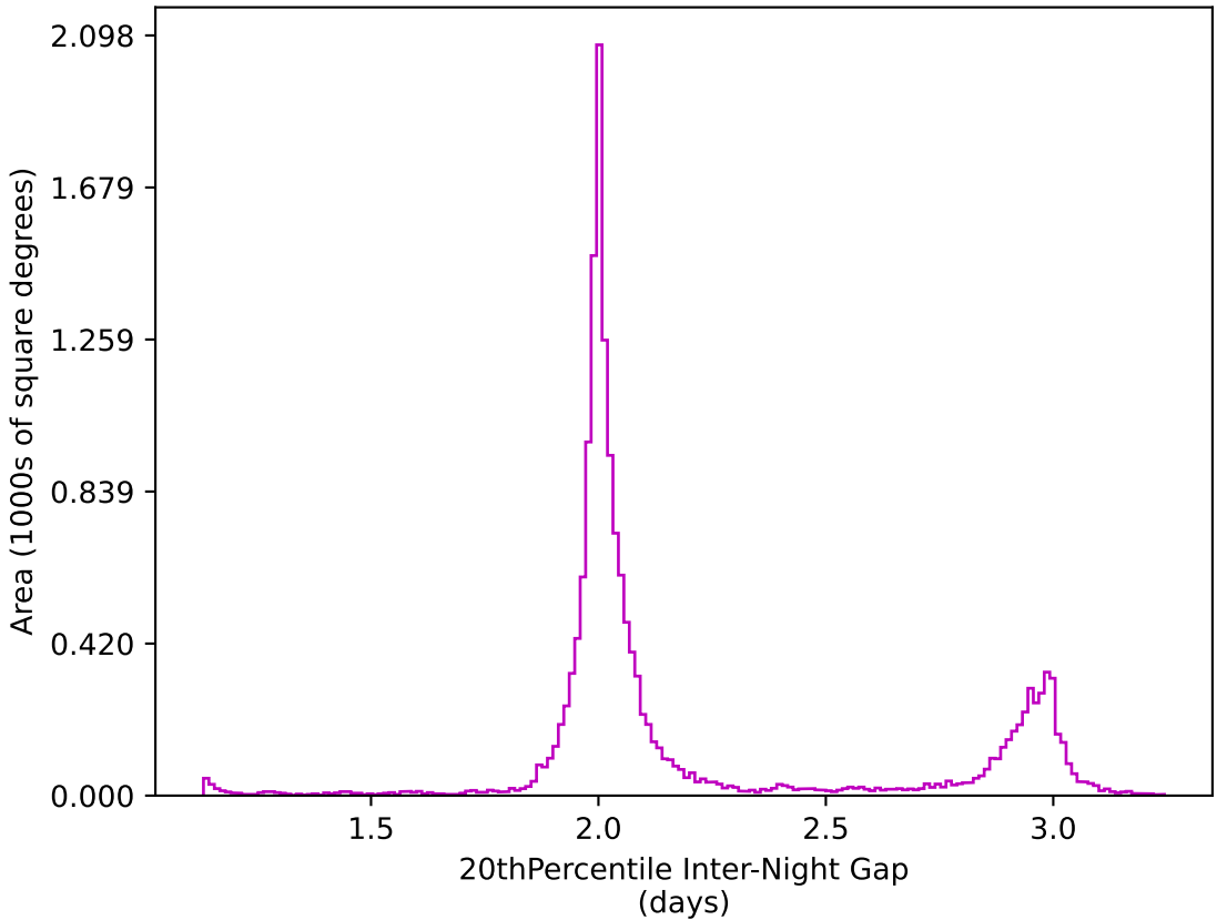
ddf_acor_sf25_lsf40_lsr10_v3.4_10yrs WFD z band: 20thPercentile Inter-Night Gap
