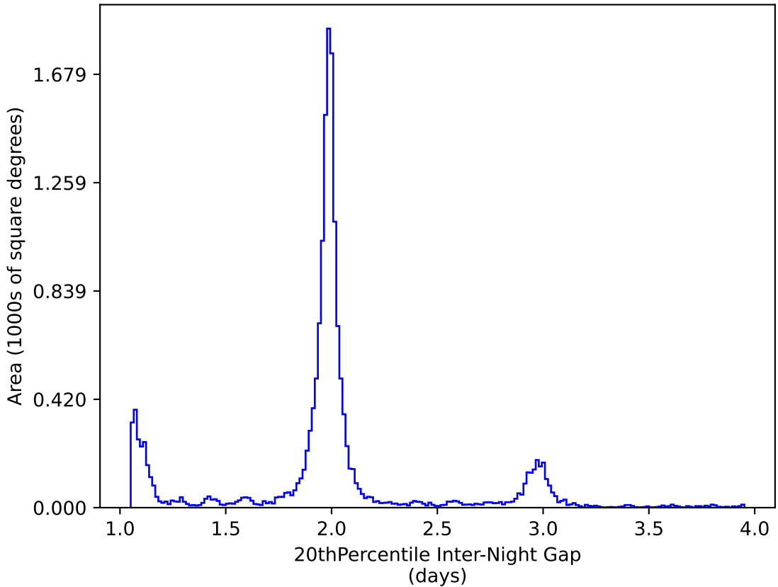
ddf_acor_sf25_lsf40_lsr10_v3.4_10yrs WFD y band: 20thPercentile Inter-Night Gap
