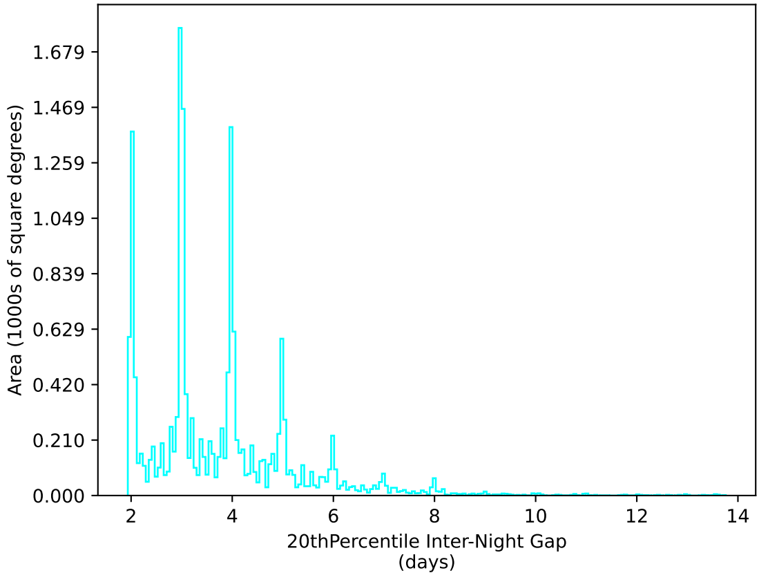
ddf_acor_sf25_lsf40_lsr10_v3.4_10yrs WFD u band: 20thPercentile Inter-Night Gap
