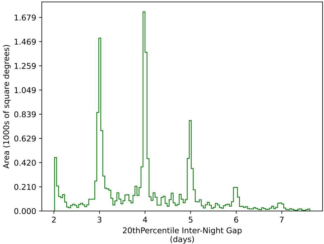
ddf_acor_sf25_lsf40_lsr10_v3.4_10yrs WFD g band: 20thPercentile Inter-Night Gap
