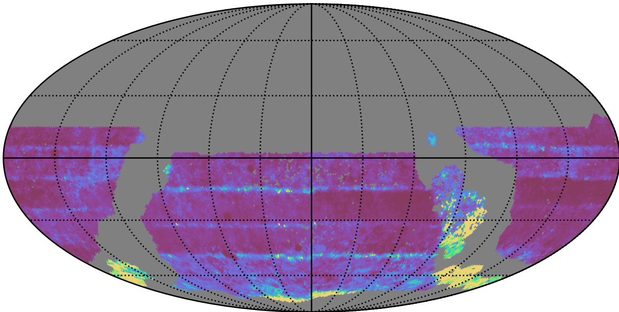
ddf_acor_sf25_lsf40_lsr10_v3.4_10yrs WFD all bands: 20thPercentile Inter-Night Gap
