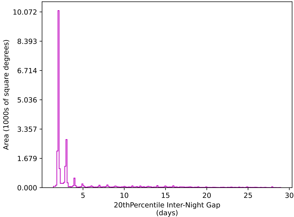
ddf_acor_sf25_lsf40_lsr10_v3.4_10yrs All sky z band: 20thPercentile Inter-Night Gap
