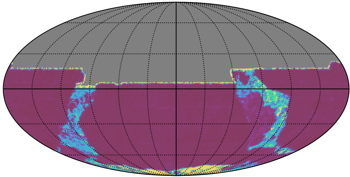
ddf_acor_sf25_lsf40_lsr10_v3.4_10yrs All sky y band: 20thPercentile Inter-Night Gap
