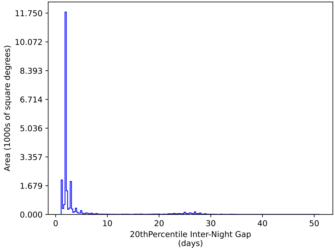
ddf_acor_sf25_lsf40_lsr10_v3.4_10yrs All sky y band: 20thPercentile Inter-Night Gap
