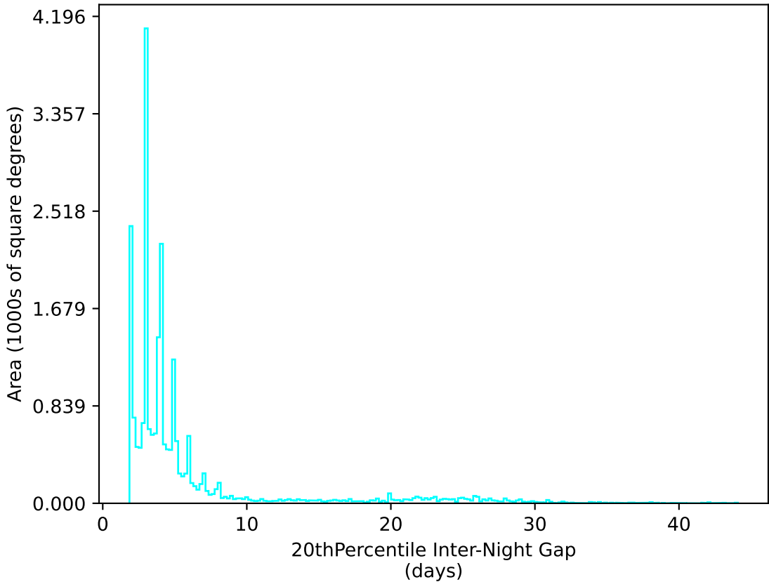
ddf_acor_sf25_lsf40_lsr10_v3.4_10yrs All sky u band: 20thPercentile Inter-Night Gap
