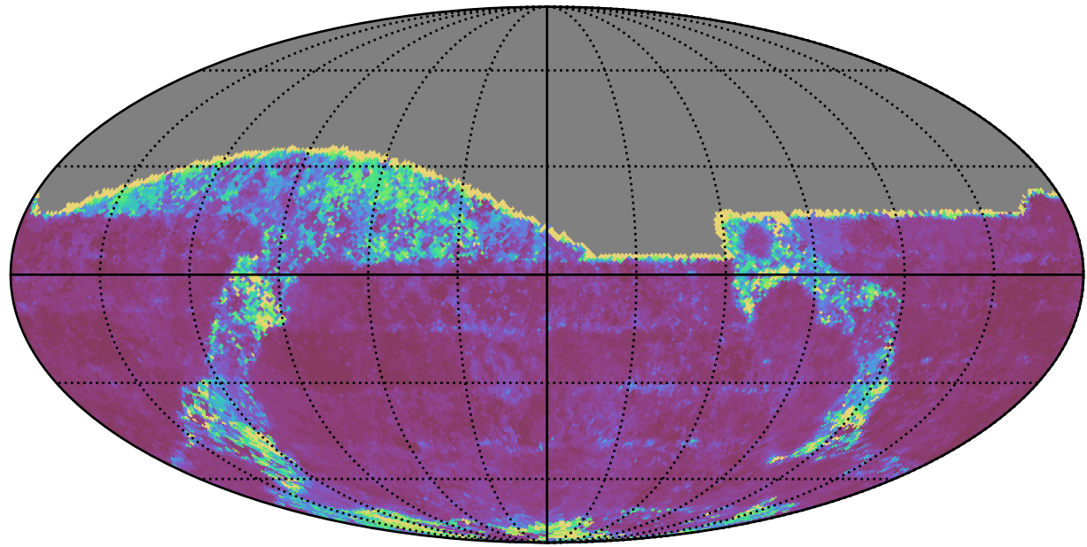
ddf_acor_sf25_lsf40_lsr10_v3.4_10yrs All sky g band: 20thPercentile Inter-Night Gap
