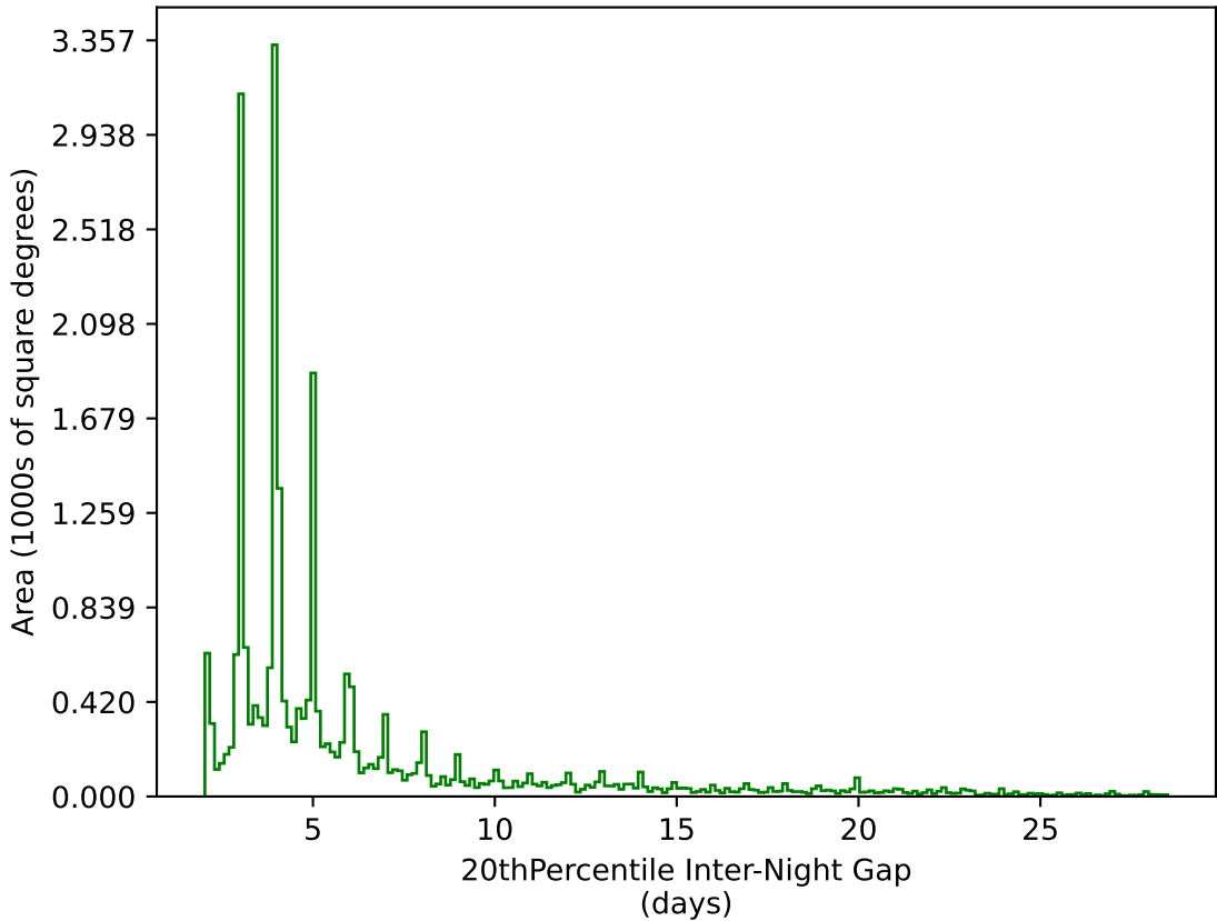
ddf_acor_sf25_lsf40_lsr10_v3.4_10yrs All sky g band: 20thPercentile Inter-Night Gap
