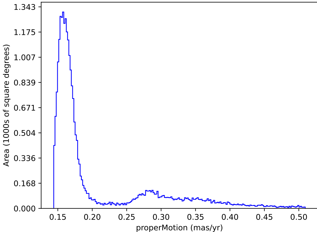
ddf_acor_sf25_ls40_lsr10_v3.4_10yrs : properMotion
