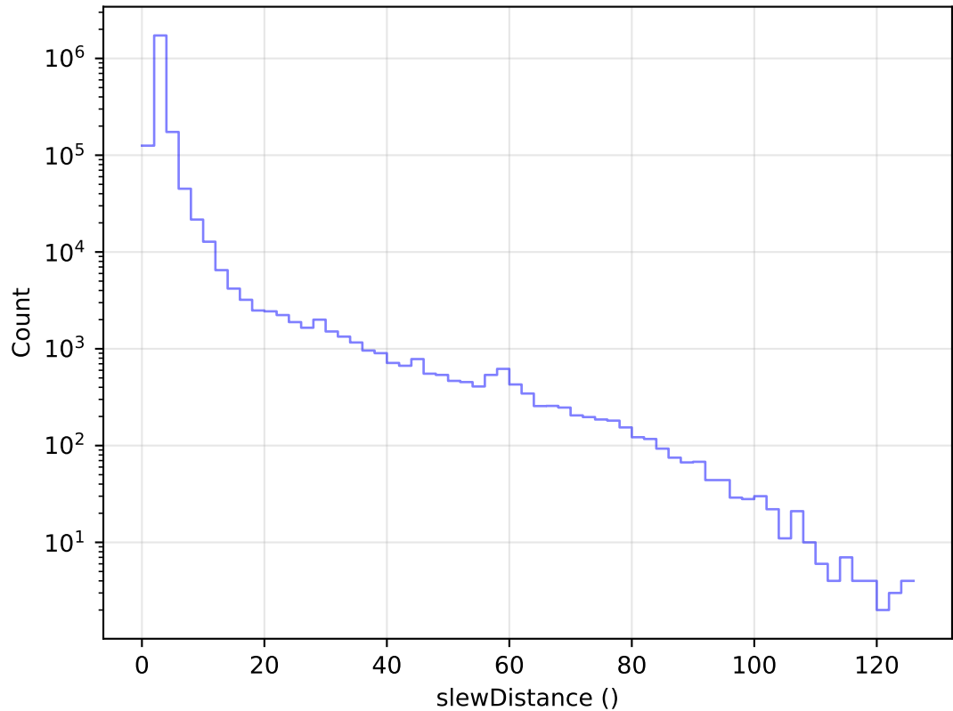
ddf_acor_sf25_lsf40_lsr10_v3.4_10yrs All visits: Slew Distance Histogram
